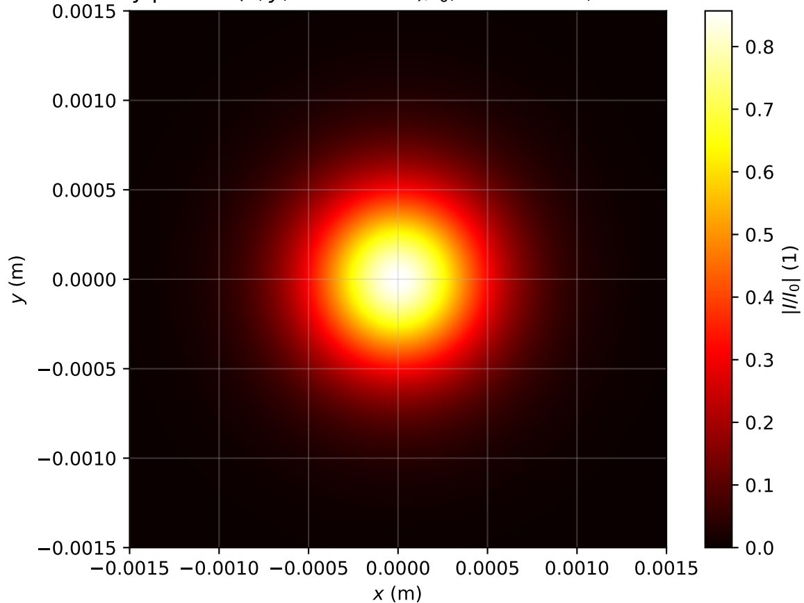
Intensity profile I(x, y, z = 2.309m)/I_0 , Pin=0.6Pcr, artificial time
